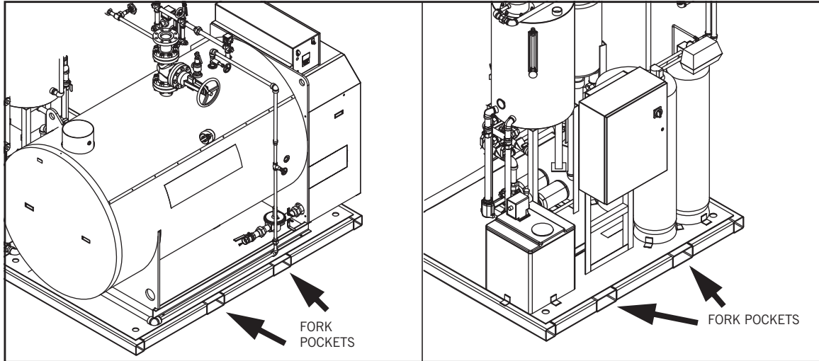
Figure 1 - Fork Lift Pockets
