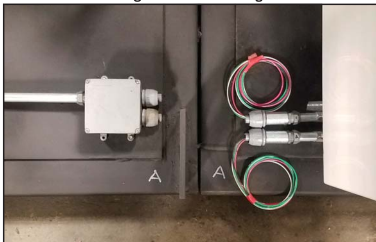
Figure 4 - Skid Wiring
