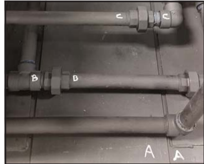
Figure 3 - Match Marks
