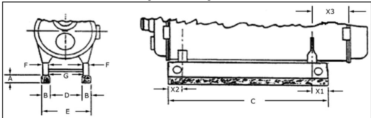
Figure 3. Mounting Piers
